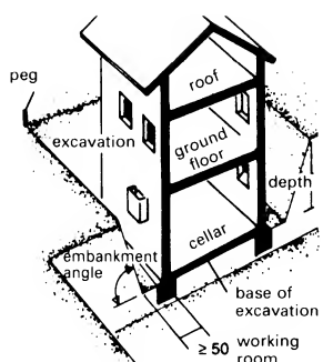
⑤ The house in the excavation
